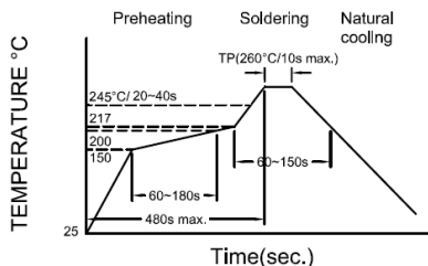
Figure 1. : Re-flow Soldering time 3 times Max.
