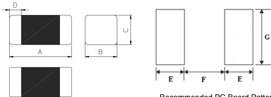
Recommended PC Board Pattern
