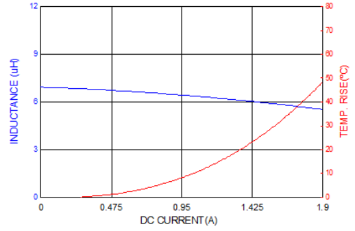
PICQ0412HP6R8MF
