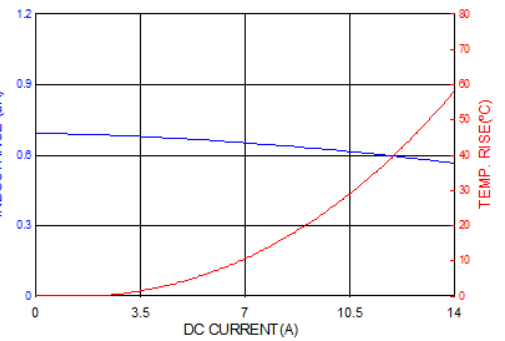
PICQ0503HR68MF
