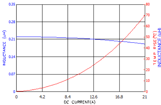
PICQ0503HR22MF
