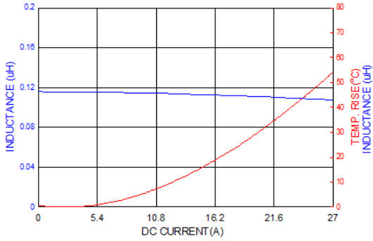
PICQ0503HR10YF
