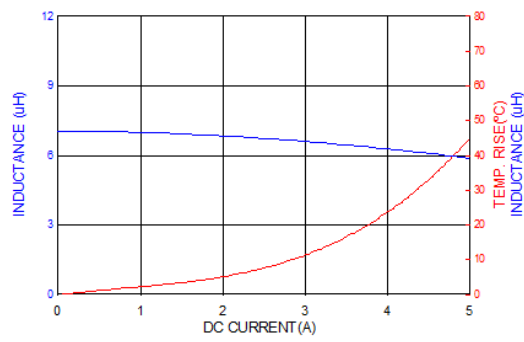
PICQ0503H6R8MF
