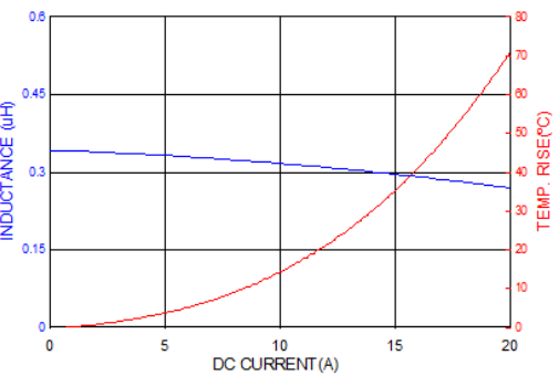
PICQ0503HR33MF
