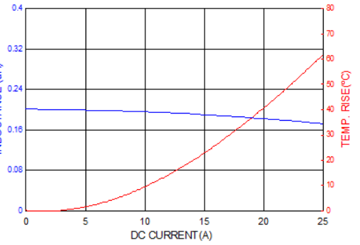
PICQ0503HR20YF
