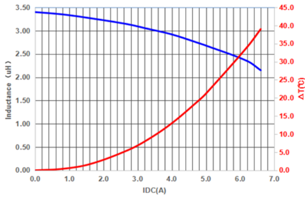
PIF0403LR3R3MN
