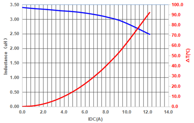
PIF0603A Series
