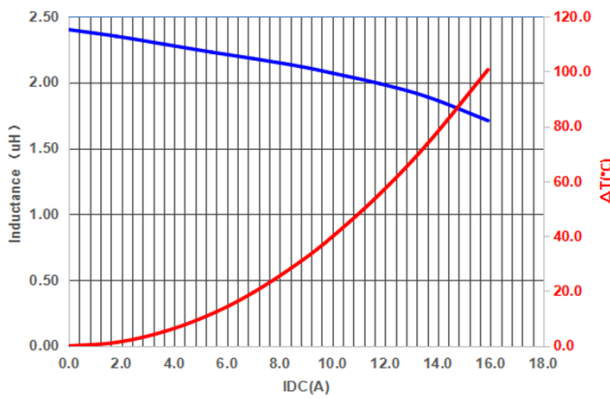
PIF0603A4R5MN
