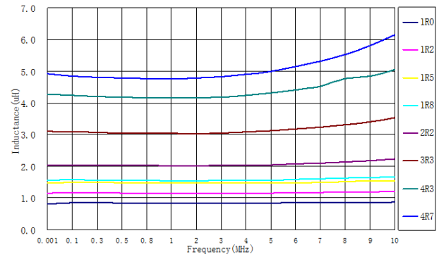
PIF0605A Series
