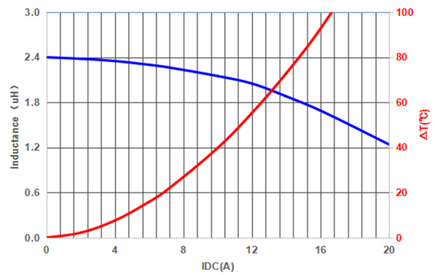
PIF0605A2R2MN
