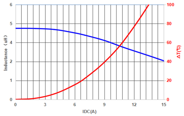
PIF0605A Series
