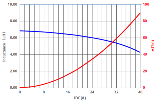
PIFQ1510A100MO
