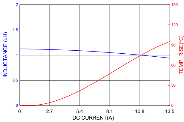
PIC0618H1R2MF
