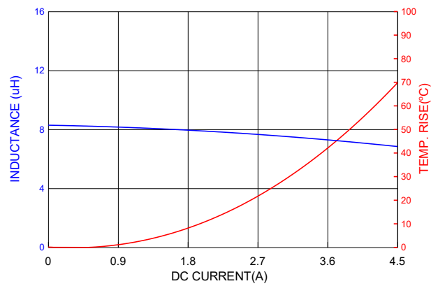
PIC0618H8R2MF
