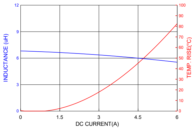
PIC0618H6R8MF
