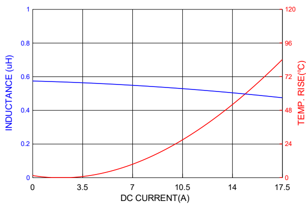
PIC0618HR56MF
