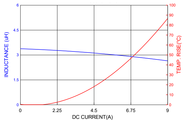
PIC0618H3R3MF
