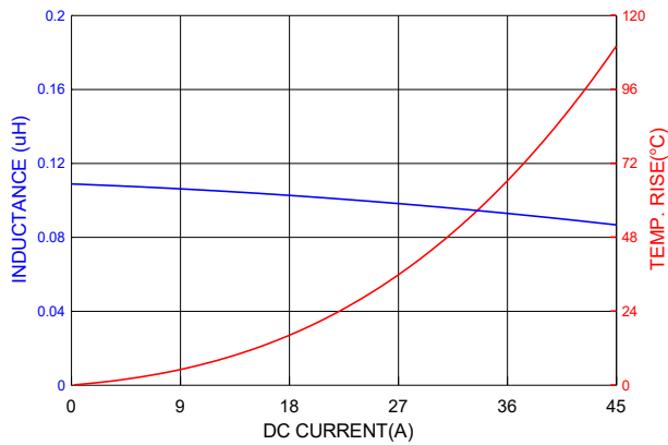
PIC0618HR10MF
