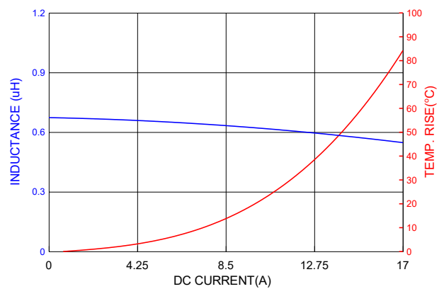
PIC0618HR68MF
