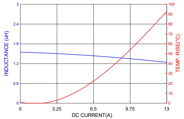
PIC0618H1R5MF
