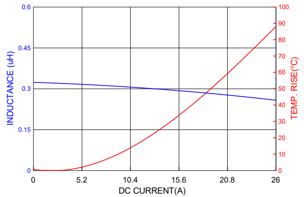
PIC0618HR22MF
