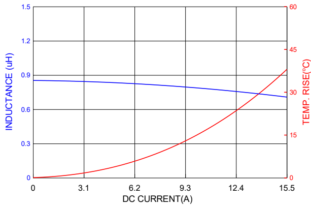
PIC0618HR82MF
