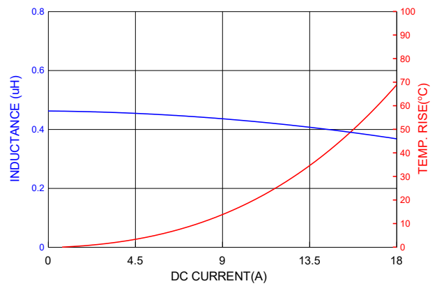
PIC0618HR47MF
