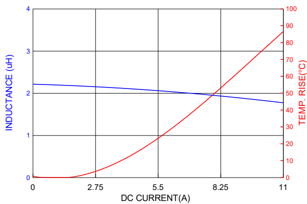
PIC0618H2R2MF
