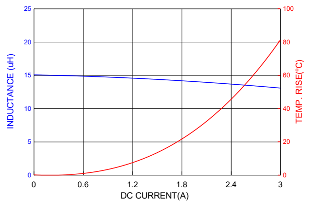
PIC0618H150MF
