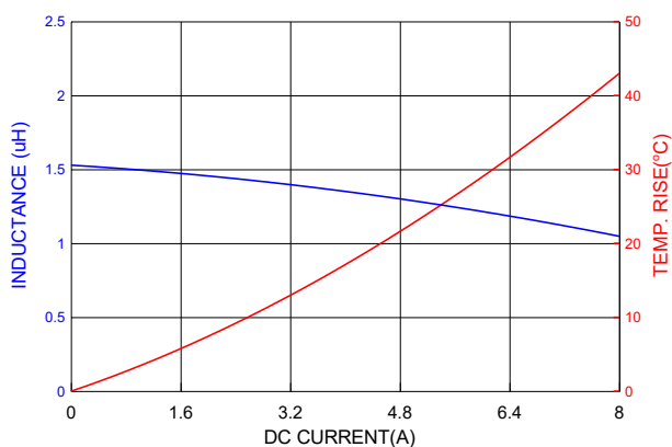
PIAQ0502SP1R5MN
