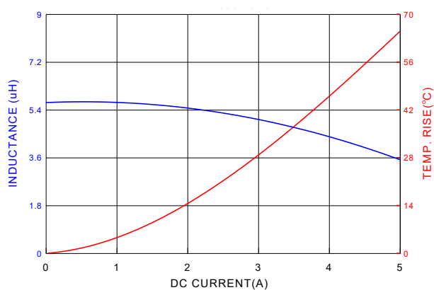
PIAQ0502SP5R6MN
