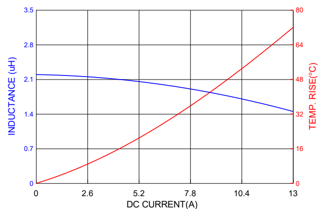
PIAQ0602S2R2MN
