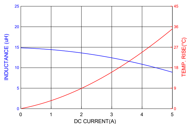
PIAQ0605S150MN
