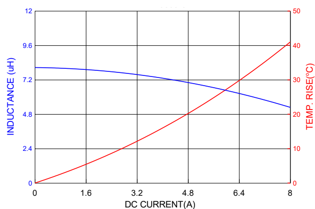
PIAQ0605S8R2MN
