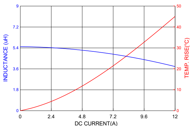
PIAQ0605S5R6MN
