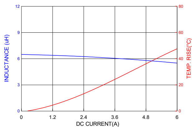
PICQ0503HP6R8MF
