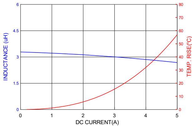
PICQ0518HP3R3MF
