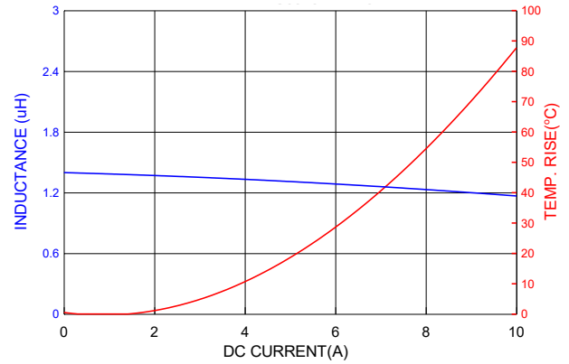
PICQ0518HP1R5MF
