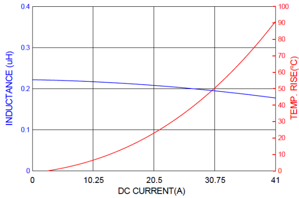
PICQ0603HR20YF
