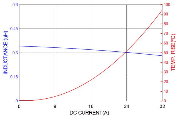
PICQ0603HR33MF
