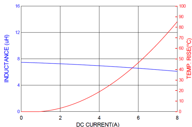
PICQ0603H6R8MF
