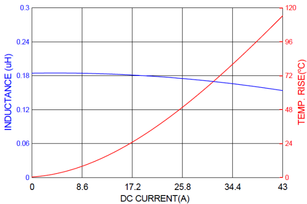
PICQ0603HR18YF
