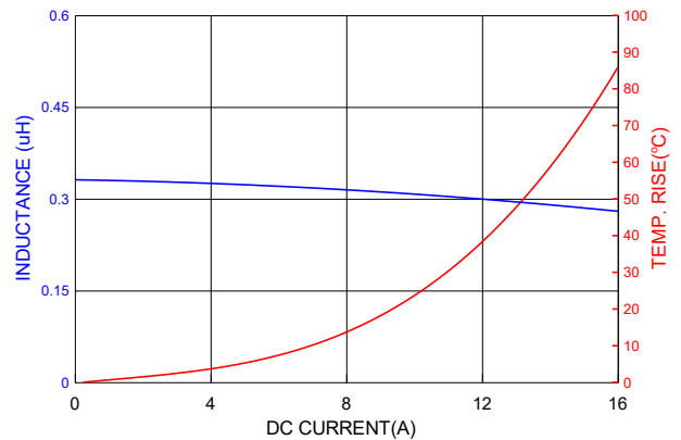
PICQ0612HR33MF
