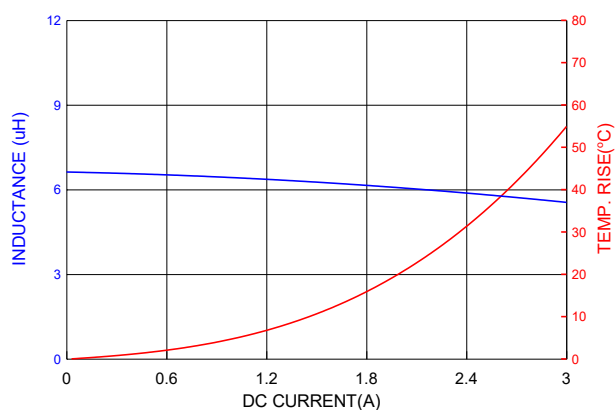
PICQ0612H6R8MF
