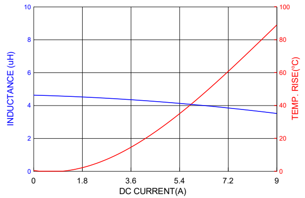
PICQ0624H4R7MF
