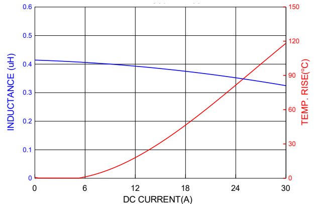
PICQ0624HR36MF
