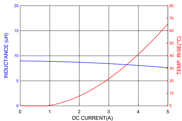
PICQ0624H100MF
