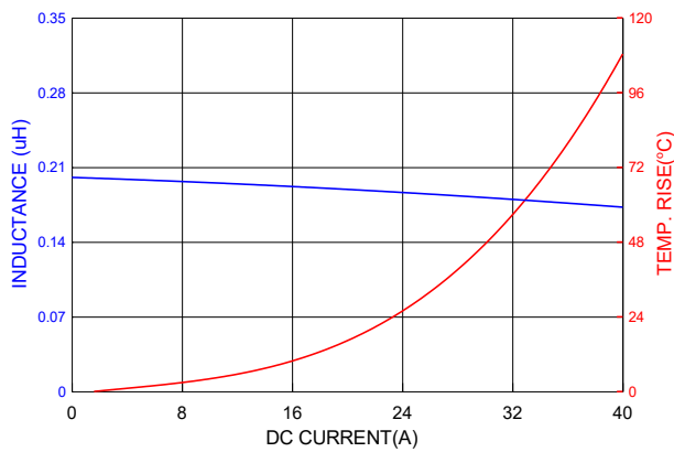
PICQ0624HR20MF
