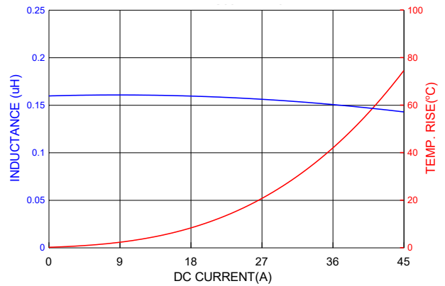
PICQ0624HR15YF
