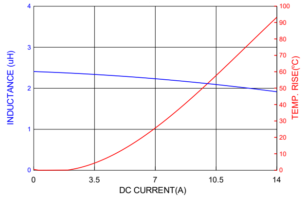
PICQ0624H2R2MF
