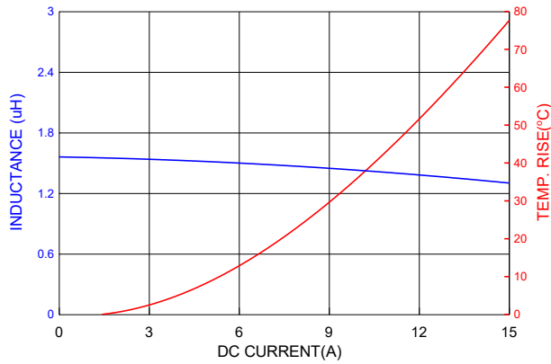
PICQ0624H1R5MF
