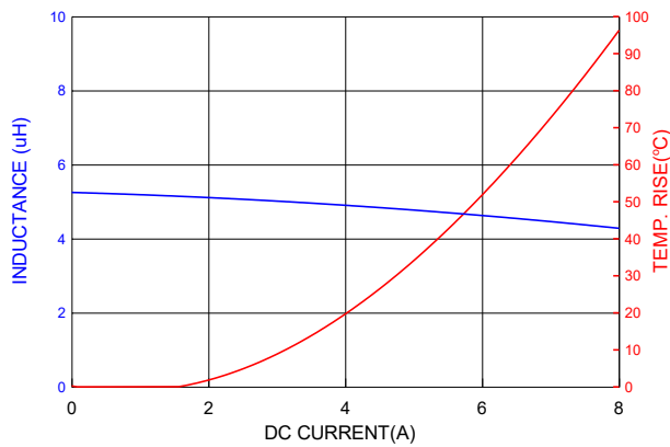
PICQ0624H5R6MF
