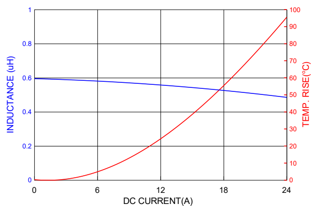
PICQ0624HR56MF
