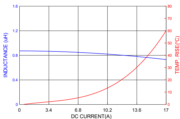
PICQ0624HR82MF
