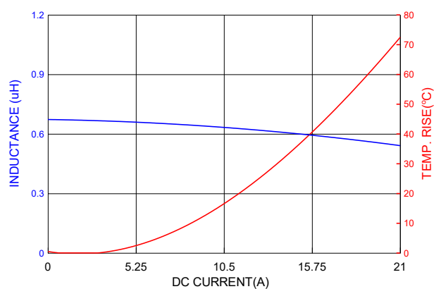
PICQ0624HR68MF
