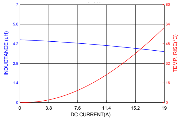
PICQ1005H4R7MF
