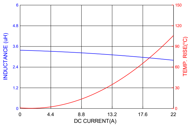
PICQ1005H3R3MF
