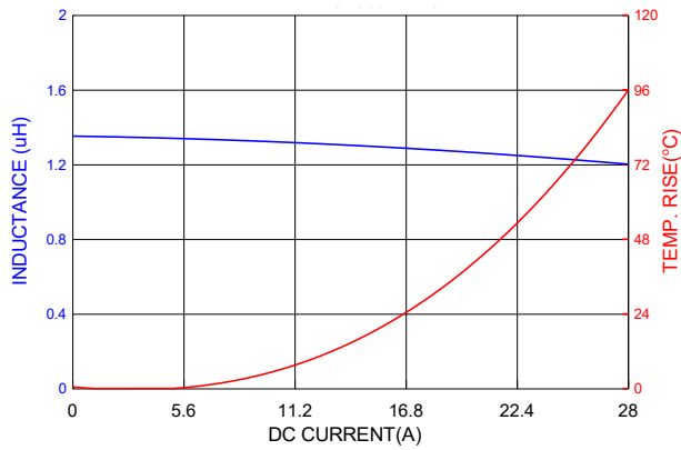
PICQ1005H1R3MF
