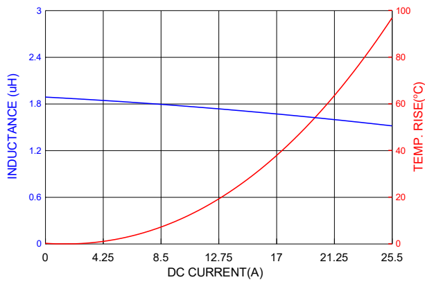
PICQ1005H1R8MF
