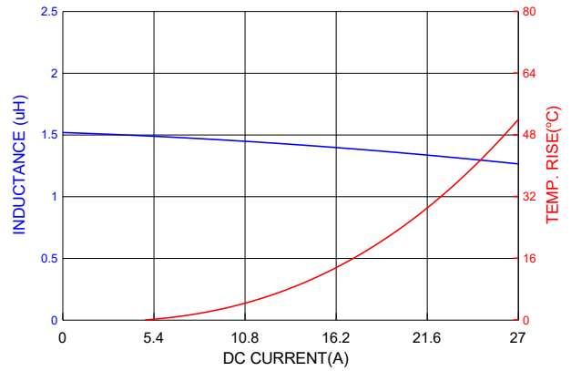
PICQ1005H1R5MF
