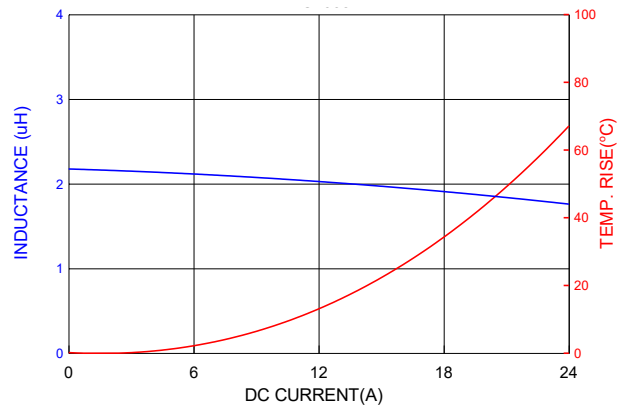
PICQ1005H2R2MF
