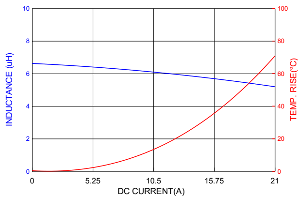
PICQ1205HP6R8MF
