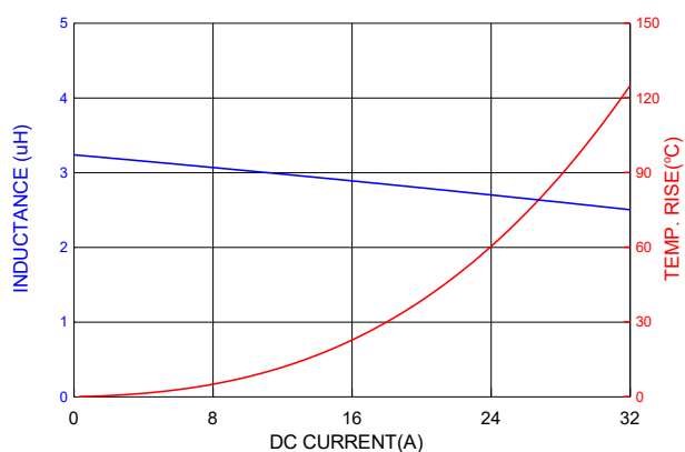
PICQ1205HP3R3MF
