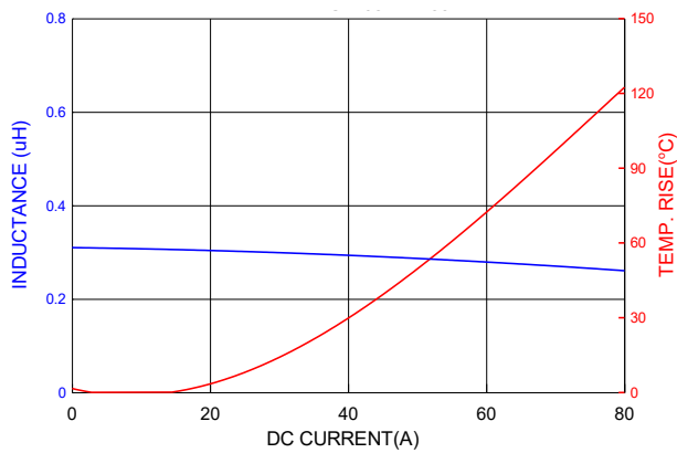
PICQ1205HPR33MF
