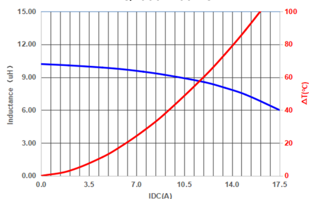
PIFQ1006A100MO
