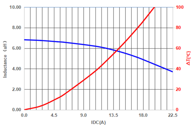
PIFQ1006A6R8MO
