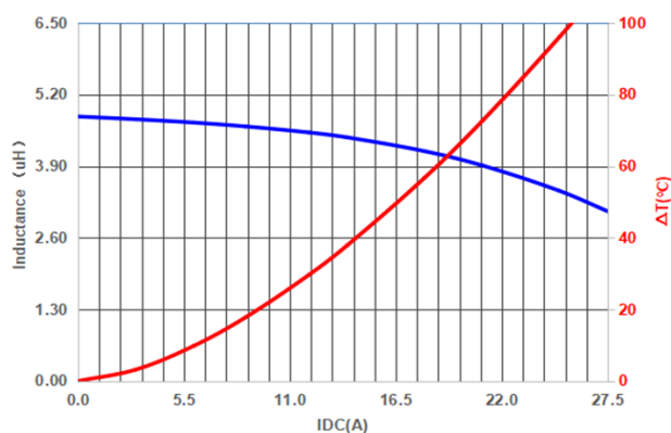
PIFQ1006A4R7MO
