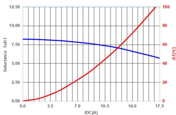
PIFQ1006A8R2MO
