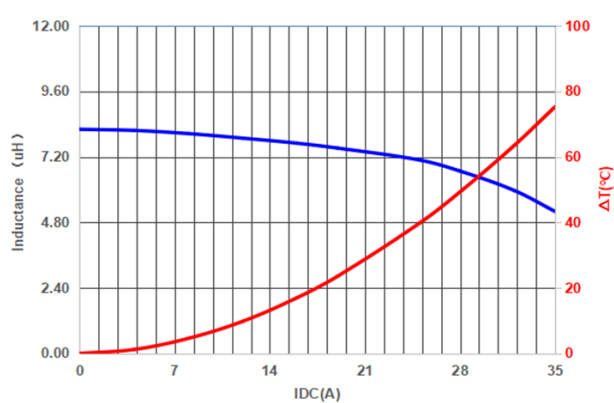
PIFQ1510A8R2MO
