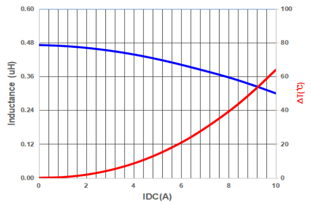
PIMQ322520AR47MN
