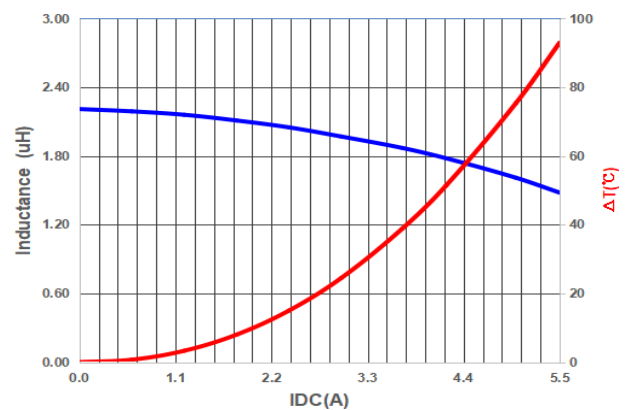
PIMQ322520A2R2MN
