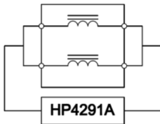
Common mode
