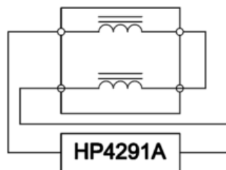
Differential mode
