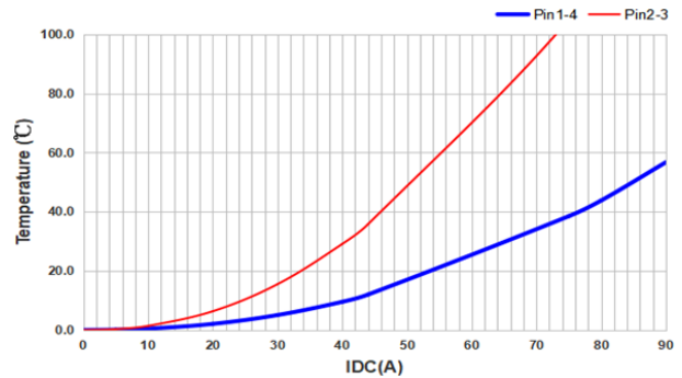
Temperature VS IDC
