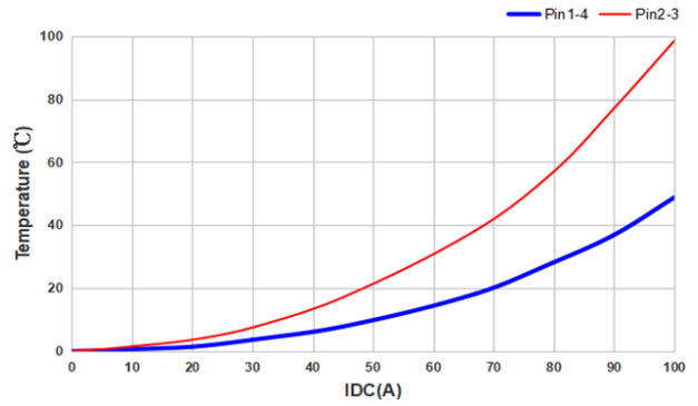
Temperature VS IDC
