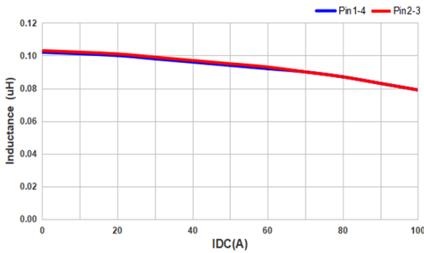
Inductance VS IDC
