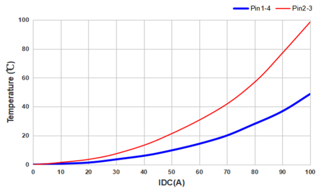
Temperature VS IDC
