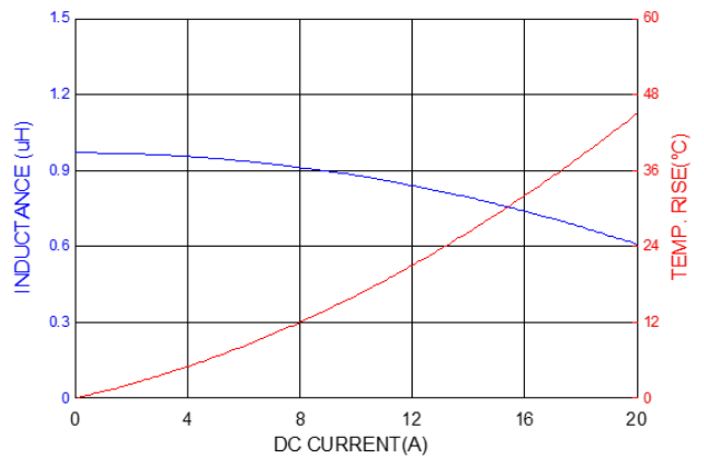
PIA0605S1R0MN
