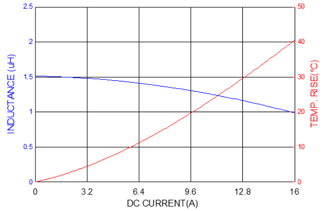
PIA0605S1R5MN
