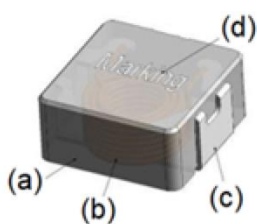
leadframe
