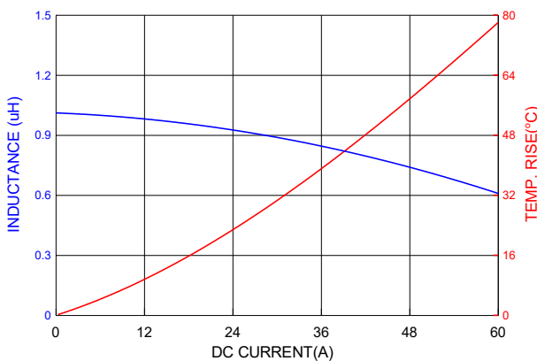
PIA1205SP1R0MN
