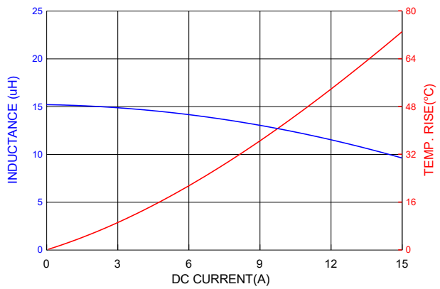
PIA1205SP150MN
