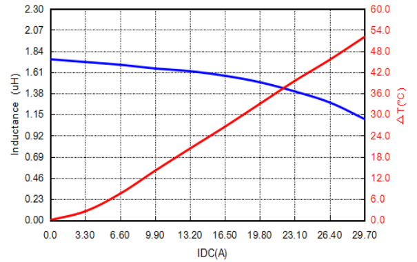
PIA1205SP1R8MN
