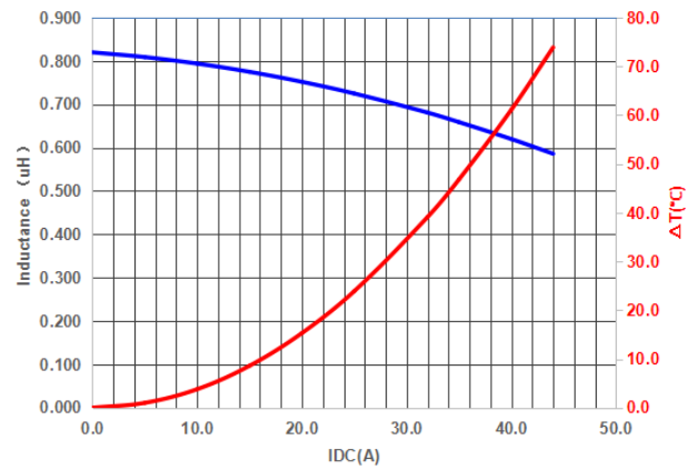
PIA1205SPR82MN
