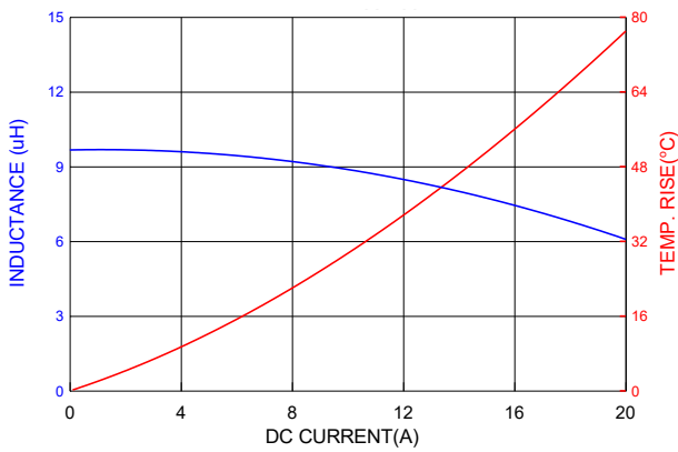
PIA1205SP100MN
