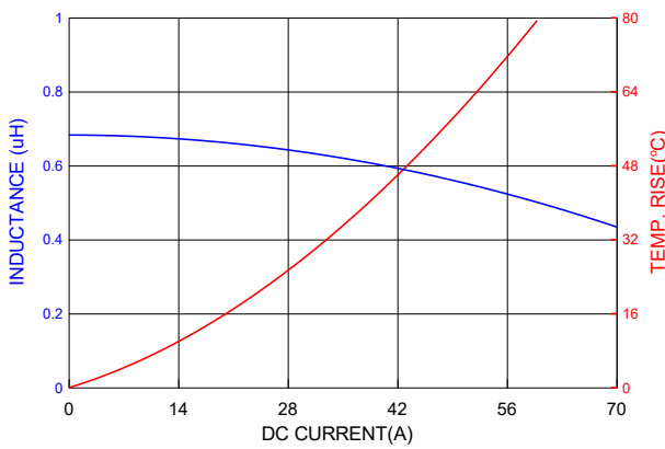
PIA1205SPR68MN
