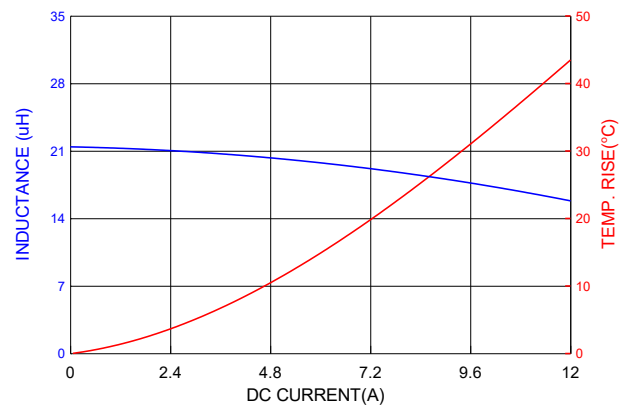
PIA1265SP220MN
