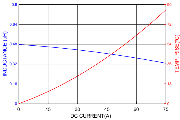
PIA1265SPR47MN
