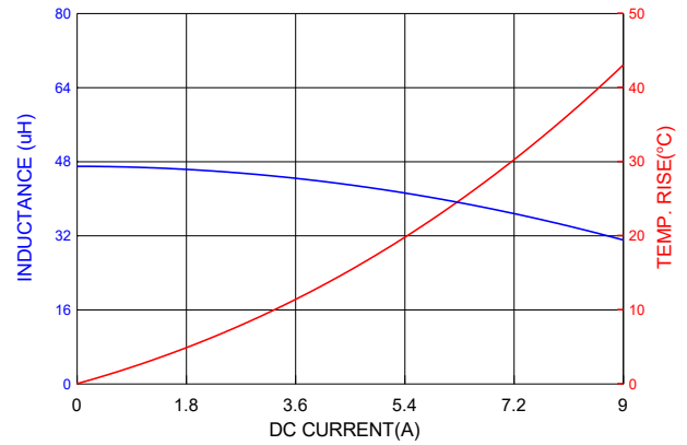
PIA1265SP470MN
