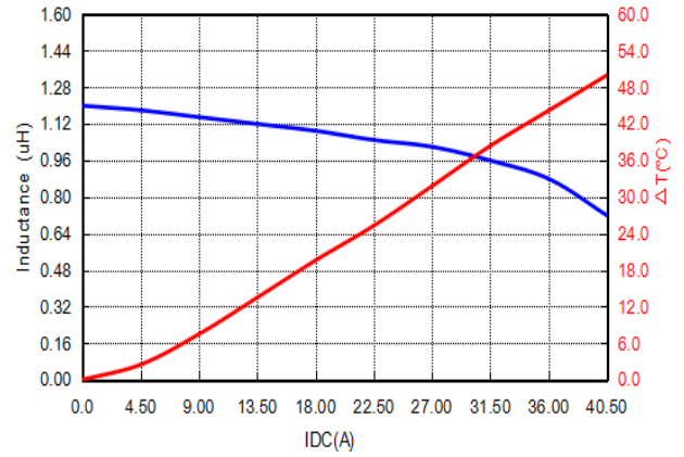
PIA1265SP1R2MN
