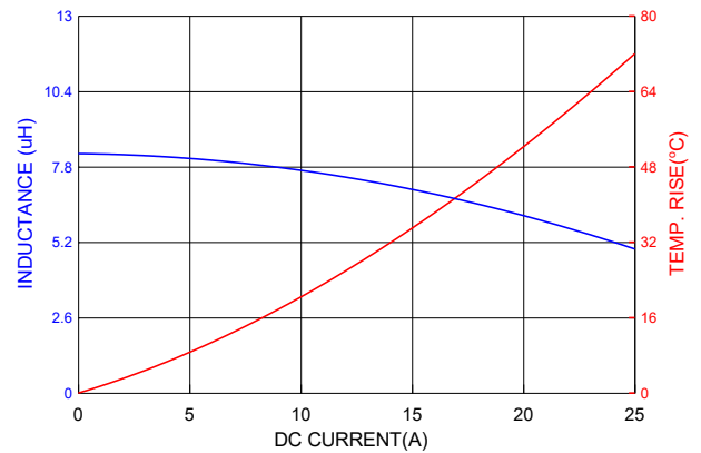
PIA1265SP8R2MN
