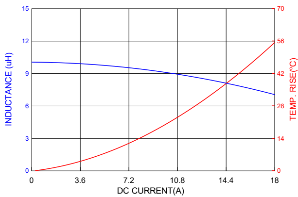
PIA1265SP100MN
