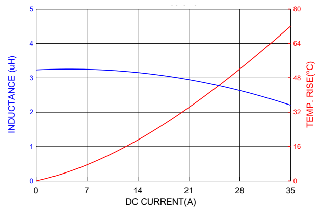
PIA1265SP3R3MN
