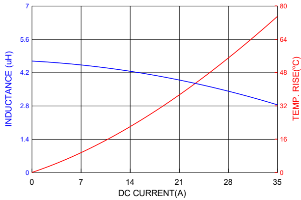
PIA1265SP4R7MN
