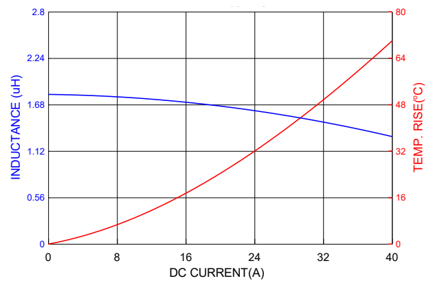
PIA1265SP1R8MN
