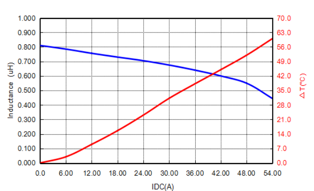
PIA1265SPR82MN
