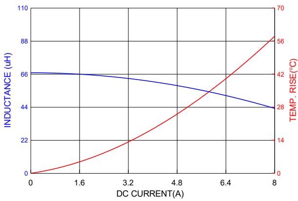
PIA1265SP680MN
