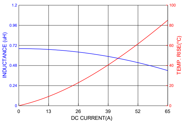
PIA1265SPR68MN
