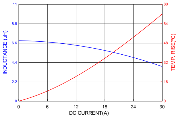
PIA1265SP6R8MN
