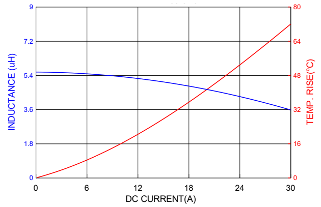
PIA1265SP5R6MN
