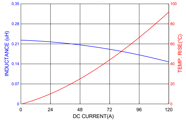
PIA1265SPR22MN
