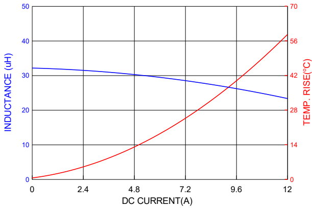
PIA1265SP330MN
