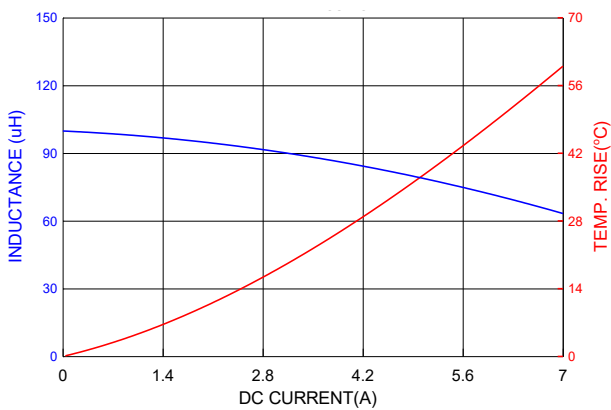
PIA1265SP101MN
