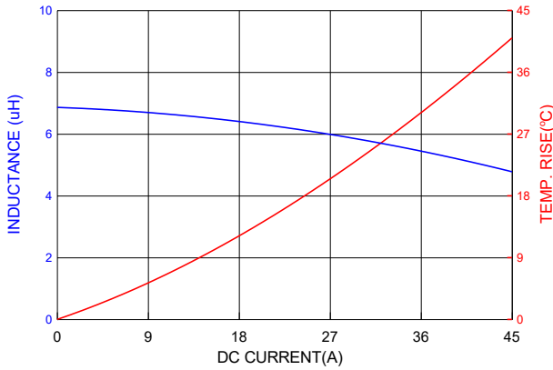
PIA2313SP6R8MN
