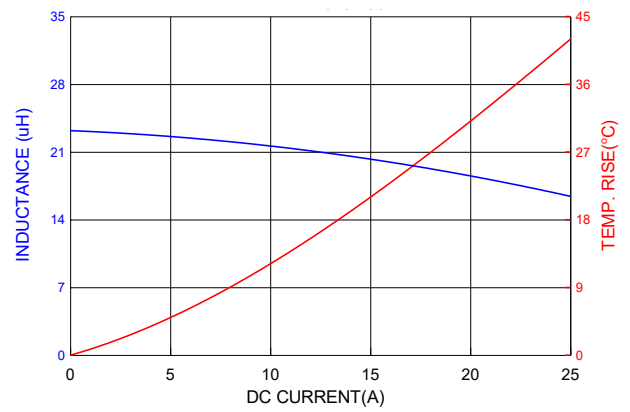
PIA2313SP230MN
