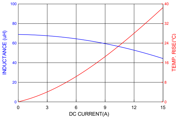
PIA2313SP680MN
