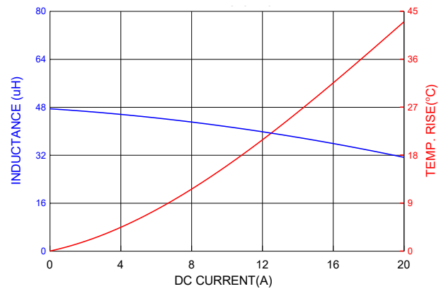
PIA2313SP470MN
