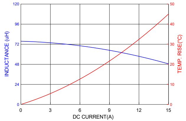
PIA2313SP750MN
