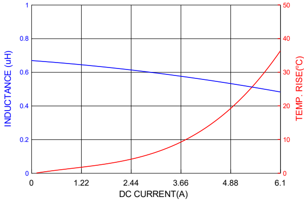
PIC0312HR68MF
