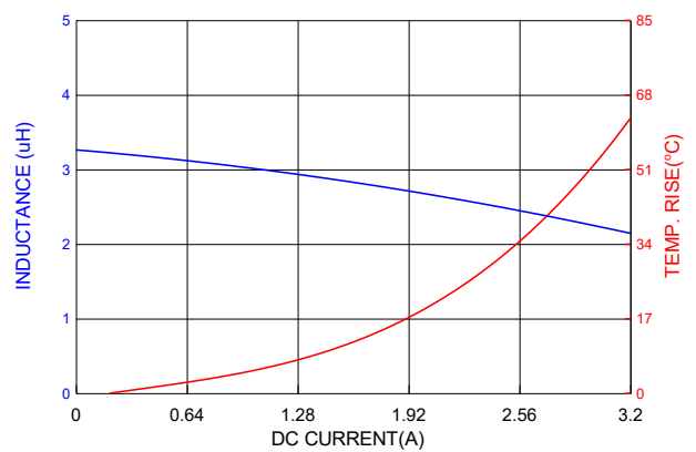
PIC0315H3R3MF
