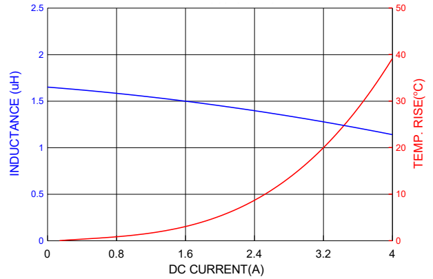
PIC0315H1R5MF
