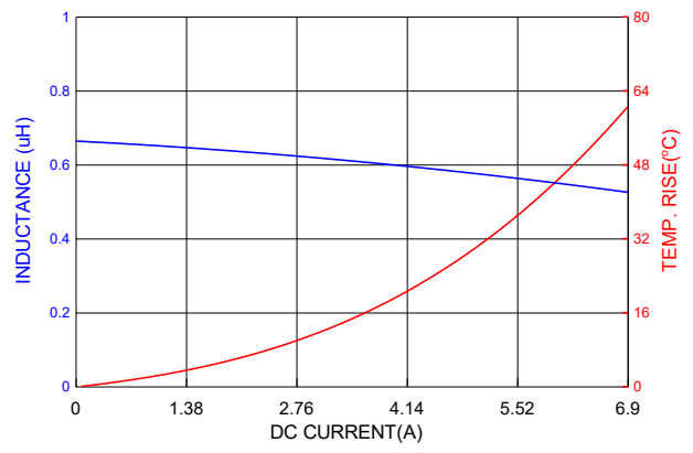
PIC0315HR68MF
