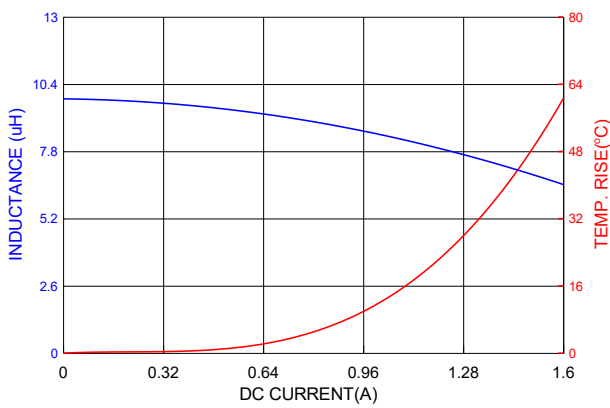
PIC0315H100MF
