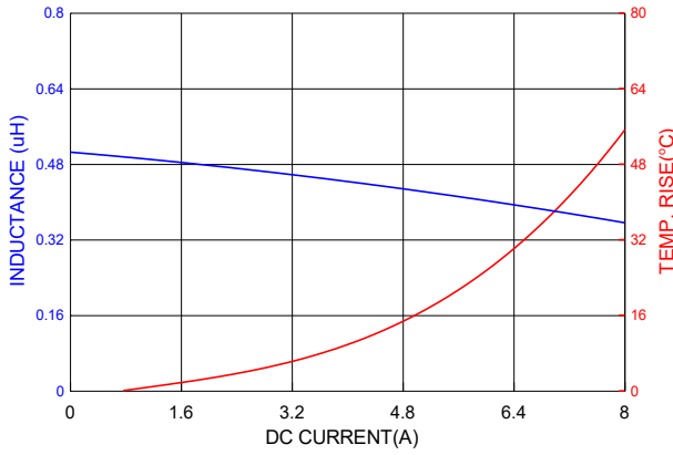
PIC0315HR47MF
