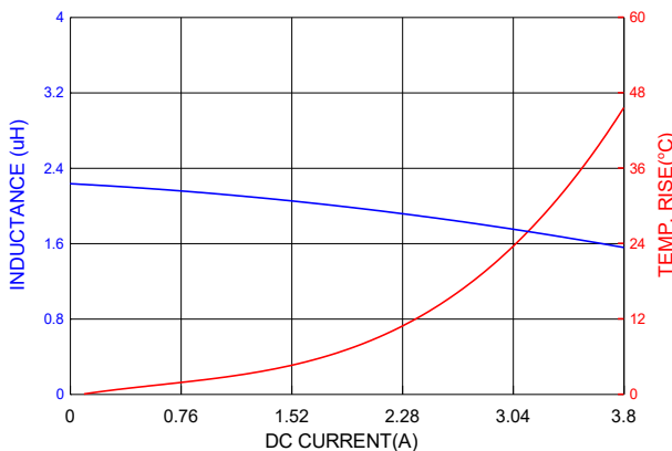
PIC0315H2R2MF
