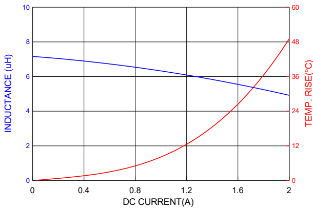
PIC0315H6R8MF
