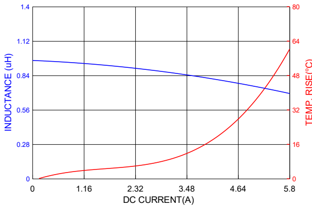
PIC0315H1R0MF
