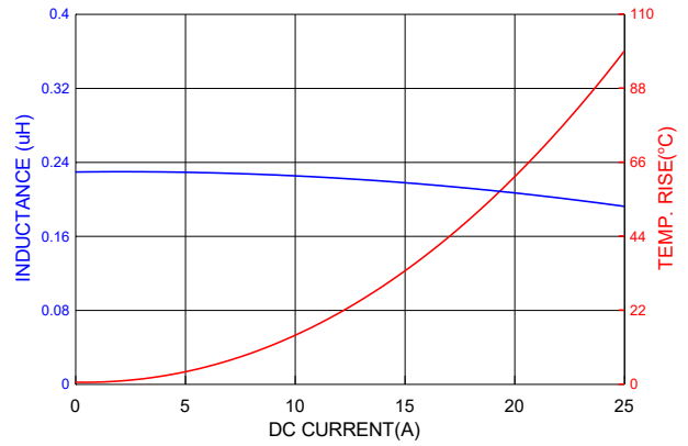
PIC0502HPR22MF
