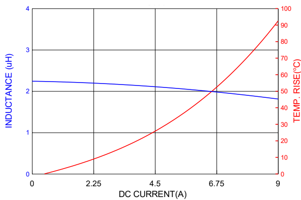
PIC0502HP2R2MF
