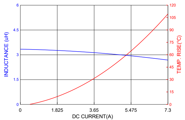
PIC0502HP3R3MF
