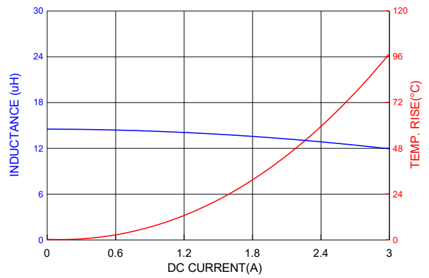
PIC0502HP150MF
