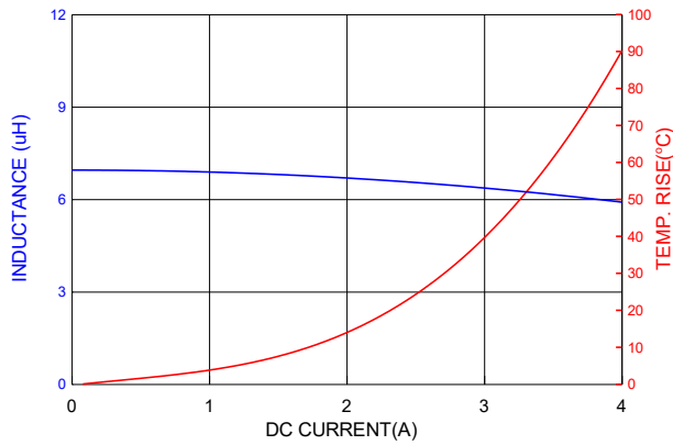
PIC0502HP6R8MF
