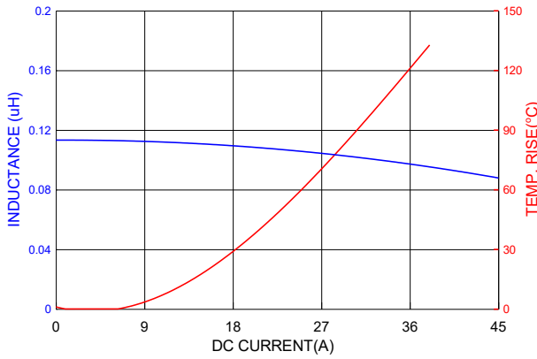
PIC0502HPR10YF
