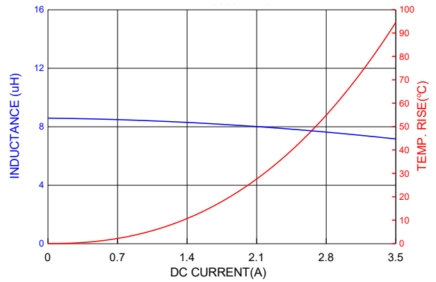
PIC0502HP8R2MF
