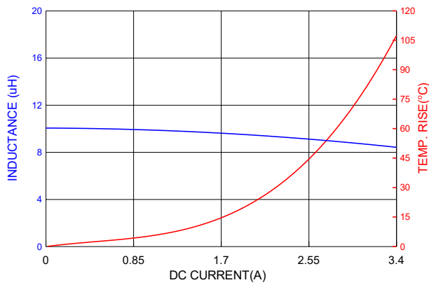
PIC0502HP100MF
