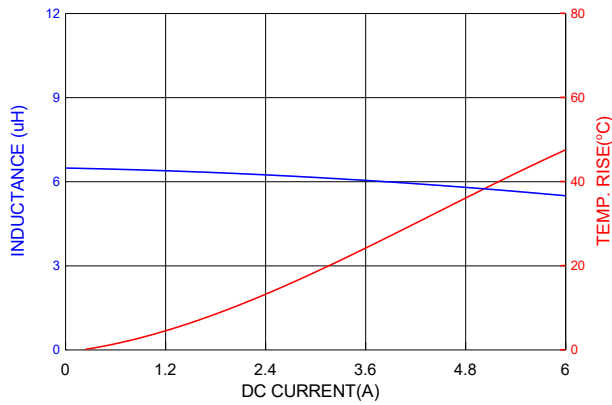
PIC0503HP6R8MF
