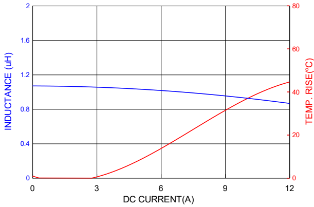
PIC0503HP1R0MF
