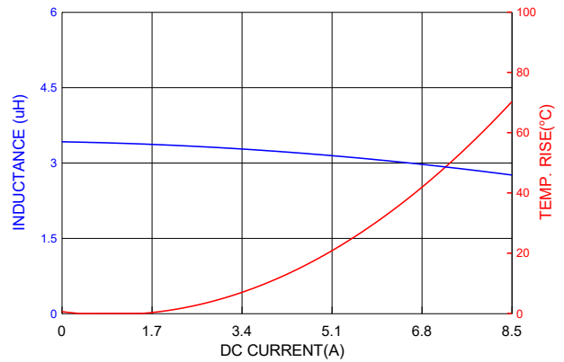
PIC0503HP3R3MF
