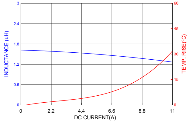
PIC0503HP1R5MF
