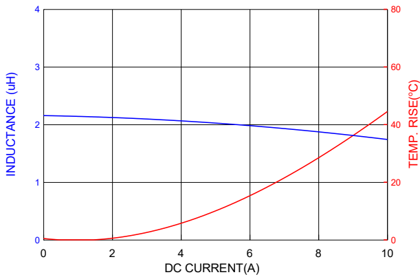
PIC0503HP2R2MF
