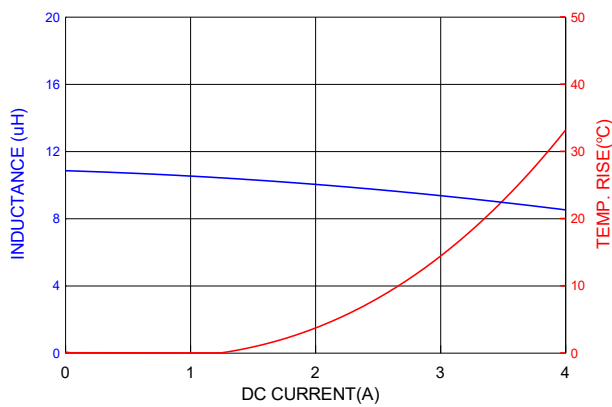
PIC0503HP100MF
