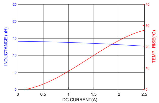
PIC0503HP150MF
