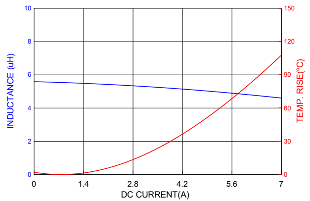
PIC0503HP5R6MF
