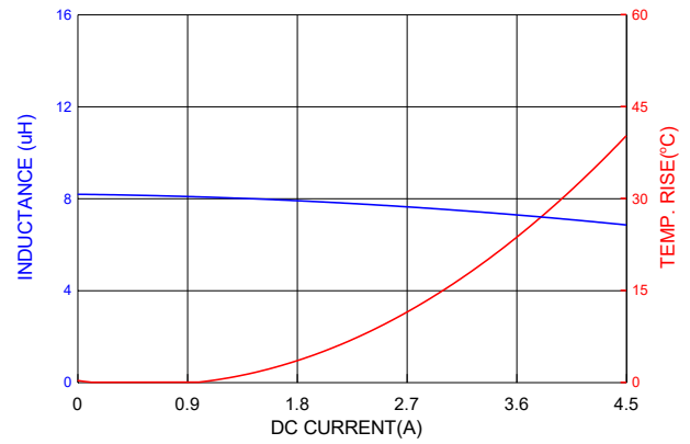
PIC0503HP8R2MF
