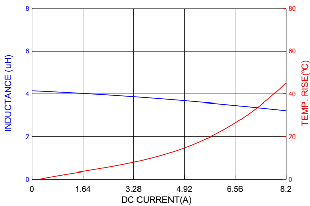
PIC0503HP4R7MF
