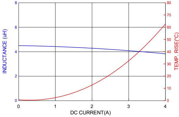
PIC0515HP4R7MF
