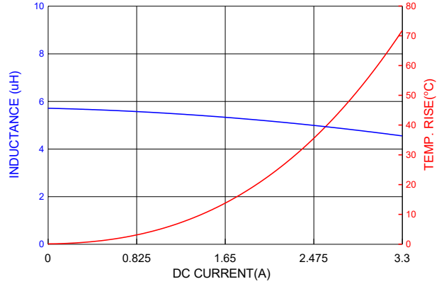
PIC0515HP5R6MF
