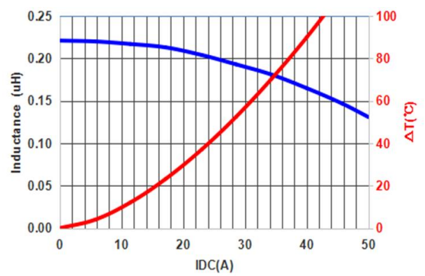
PIC0603HR22YF
