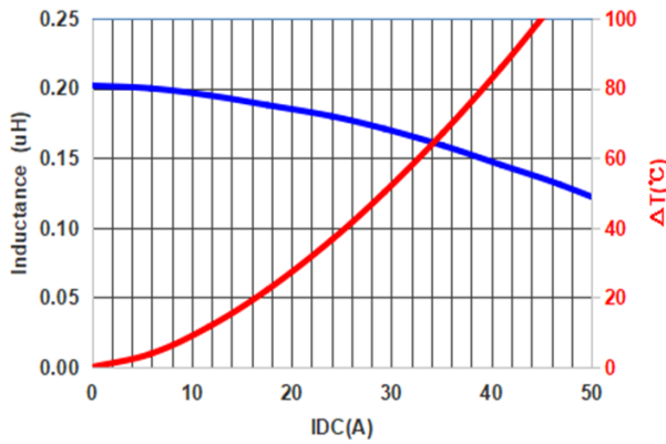
PIC0603HR20YF
