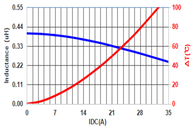
PIC0603HR40MF
