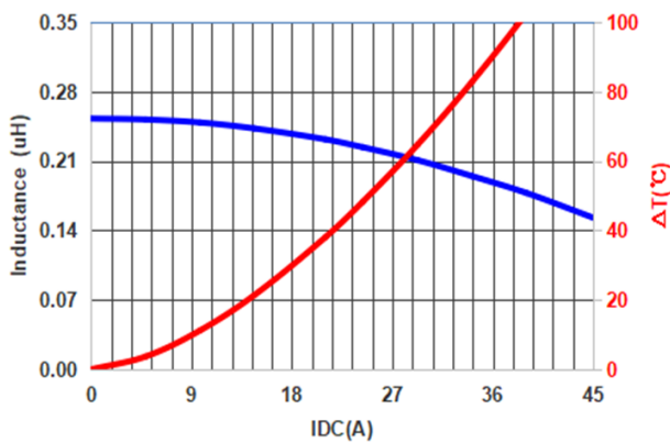
PIC0603HR25MF
