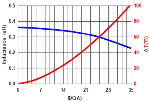
PIC0603HR36MF
