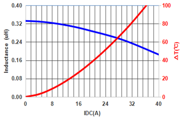
PIC0603HR33MF
