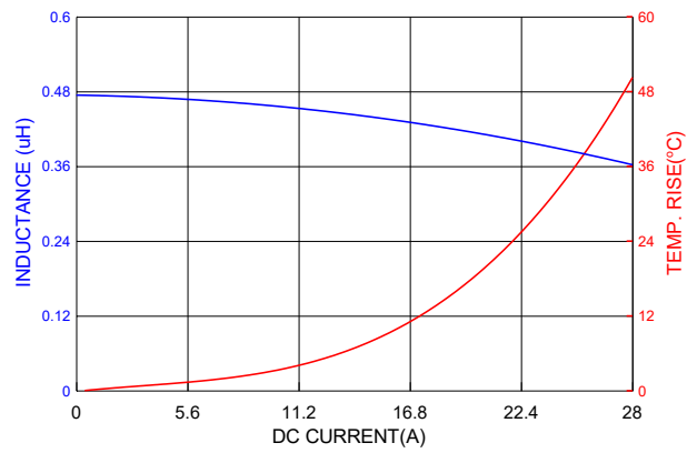
PIC0604HR47MF
