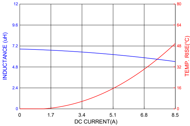
PIC0604H6R8MF
