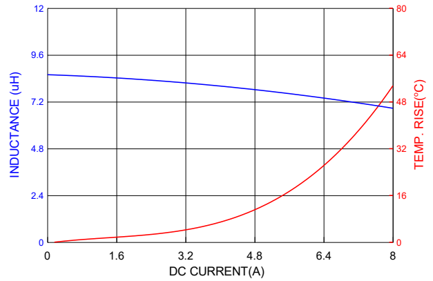
PIC0604H8R2MF
