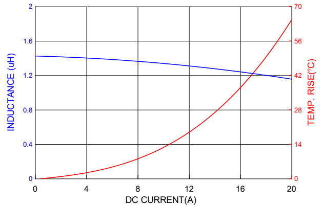
PIC0604H1R5MF
