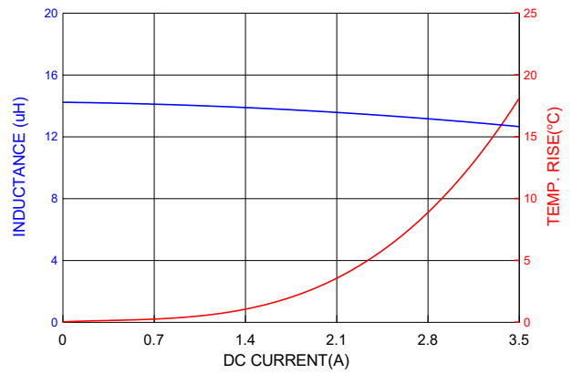
PIC0604H150MF
