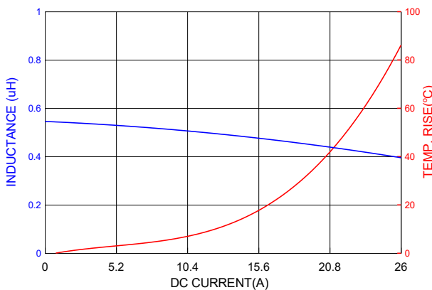
PIC0604HR56MF
