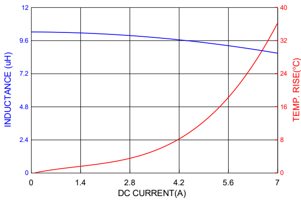
PIC0604H100MF
