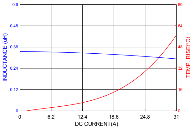
PIC0604HR36MF
