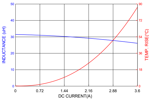
PIC0604H330MF
