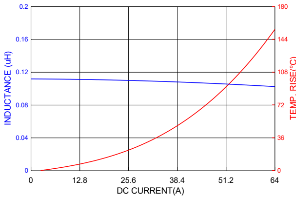
PIC0604HR12YF
