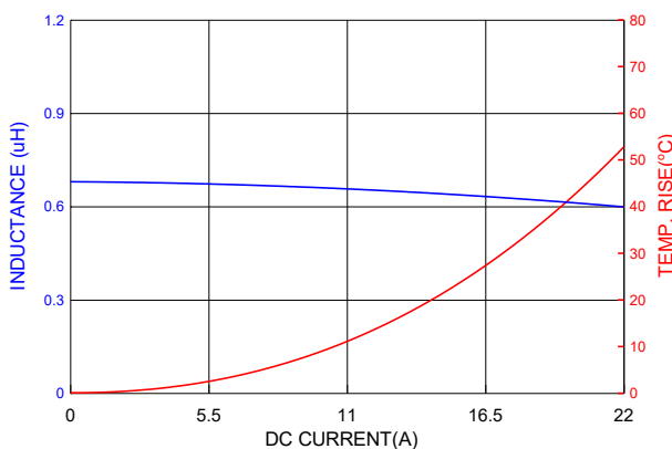
PIC0605HR68MF
