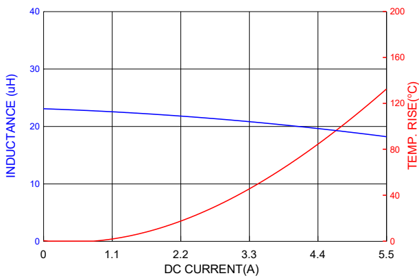
PIC0605H220MF
