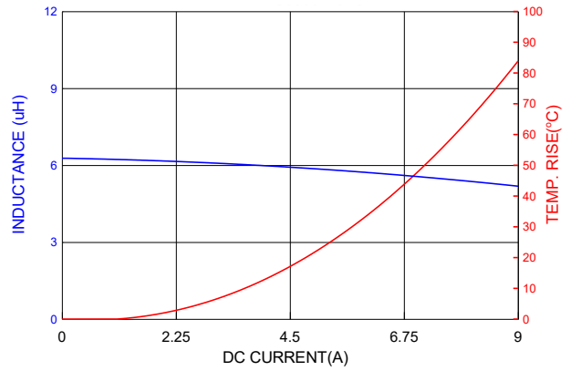
PIC0605H6R8MF
