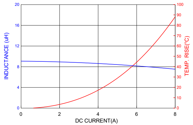
PIC0605H100MF
