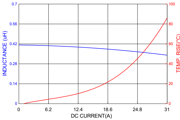
PIC0605HR40MF
