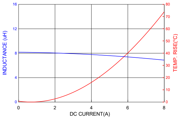
PIC0605H8R2MF
