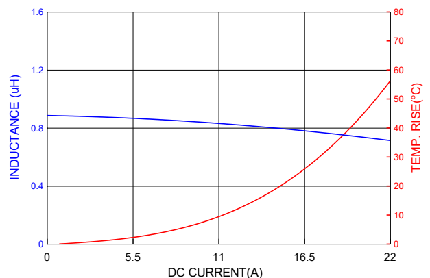
PIC0605HR82MF
