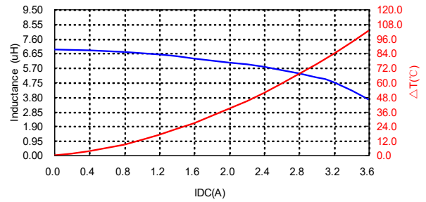
PIC0612H6R8MF
