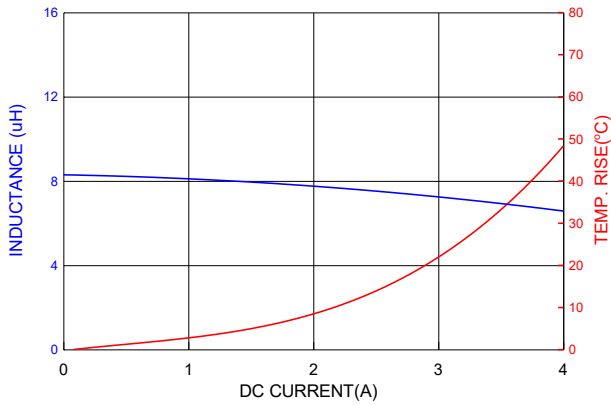
PIC0615H8R2MF
