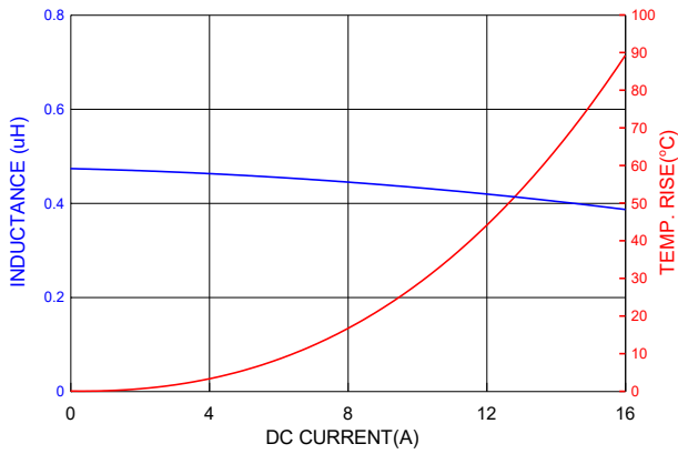
PIC0615HR47MF
