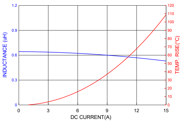
PIC0615HR68MF
