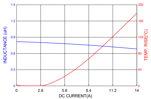
PIC0615HR82MF
