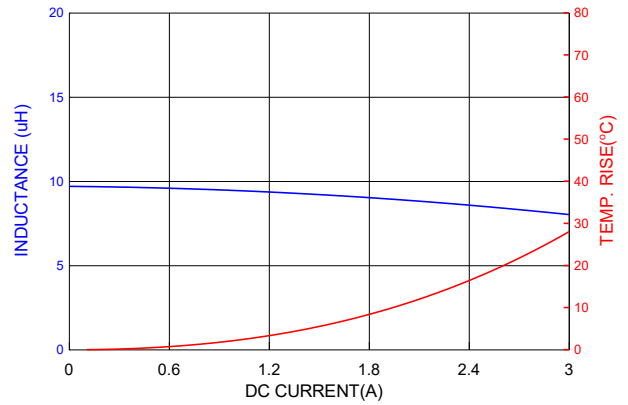
PIC0615H100MF
