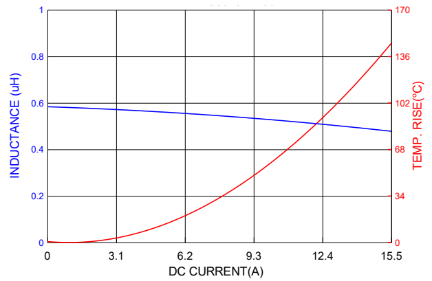
PIC0615HR56MF
