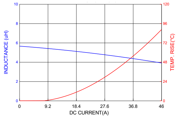
PIC1707HP5R6MF
