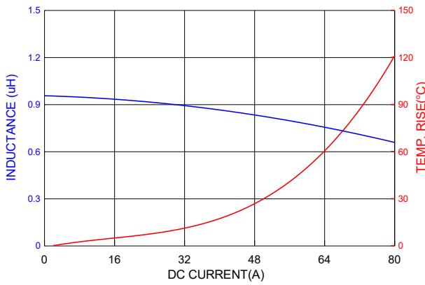
PIC1707HP1R0MF
