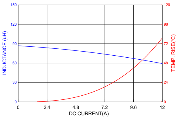
PIC1707HP101MF
