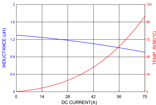
PIC1707HP1R5MF
