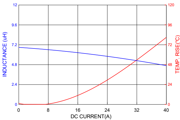
PIC1707HP6R8MF
