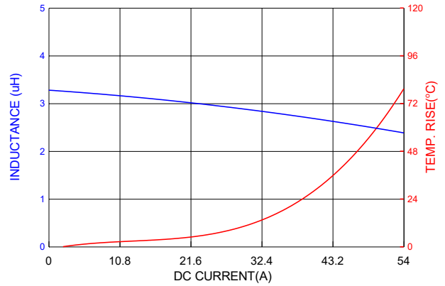
PIC1707HP3R3MF
