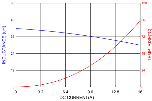
PIC1707HP470MF
