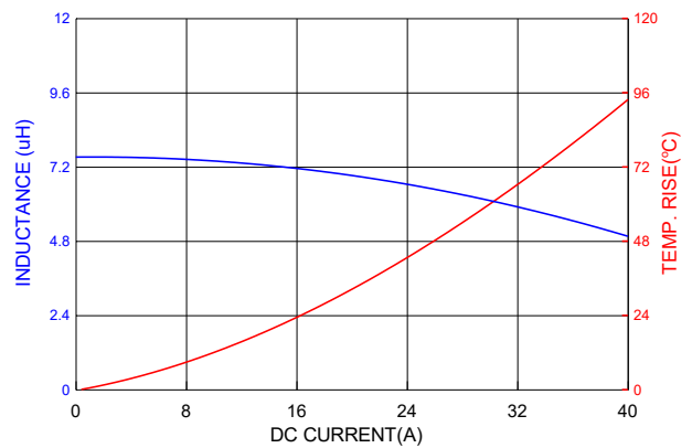
PIC1707HP7R4MF
