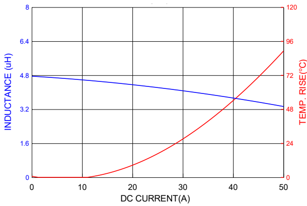
PIC1707HP4R7MF
