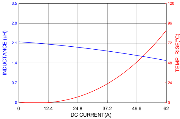
PIC1707HP2R2MF
