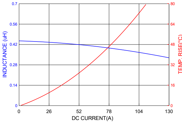
PIC1707HPR45MF
