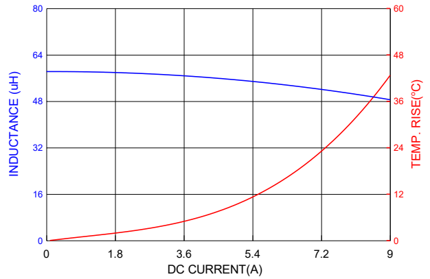
PIC1707HP560MF
