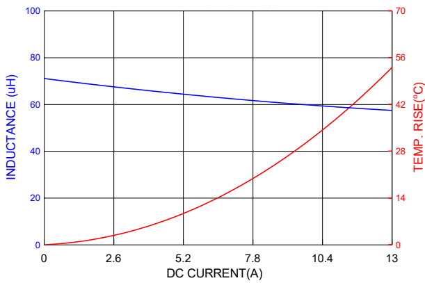
PIC1707HP680MF
