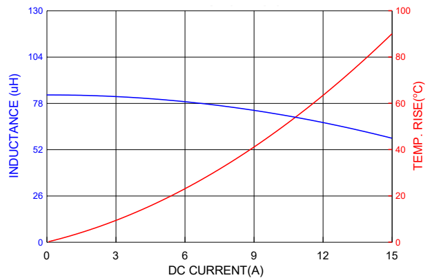
PIC1707HP820MF
