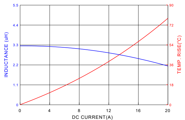
PIF0703A3R3MN
