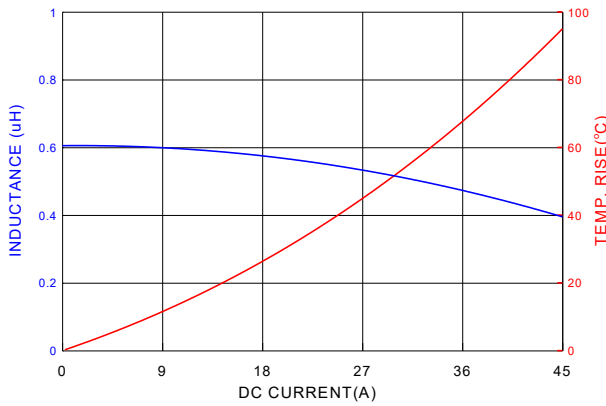
PIF0703AR60MN
