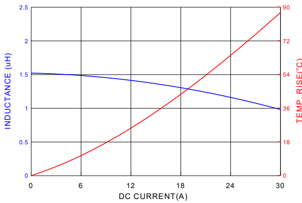
PIF0703A1R5MN
