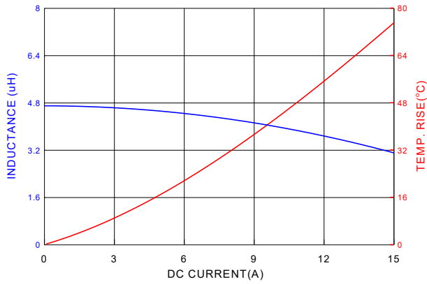
PIF0703A4R7MN
