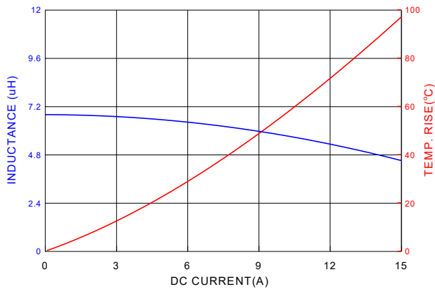
PIF0703A6R8MN
