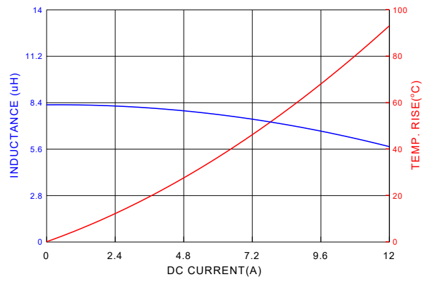
PIF0703A8R2MN
