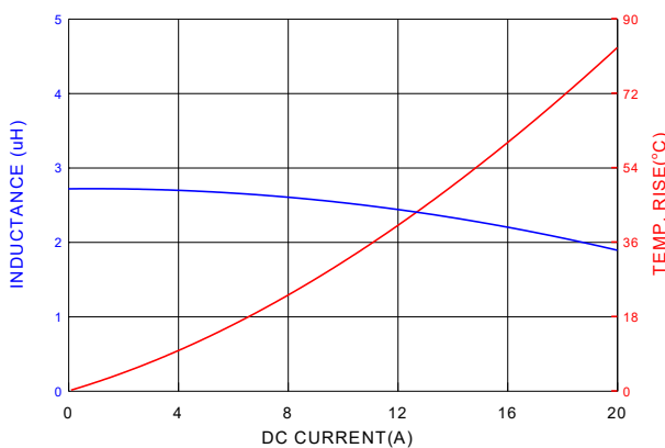
PIF0703A2R7MN
