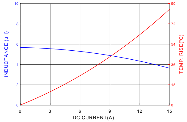
PIF0703A5R6MN
