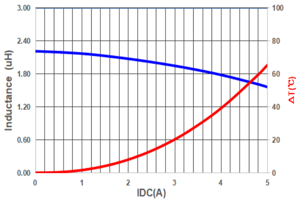
PIM322512A2R2M
