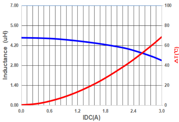
PIM322512A4R7M
