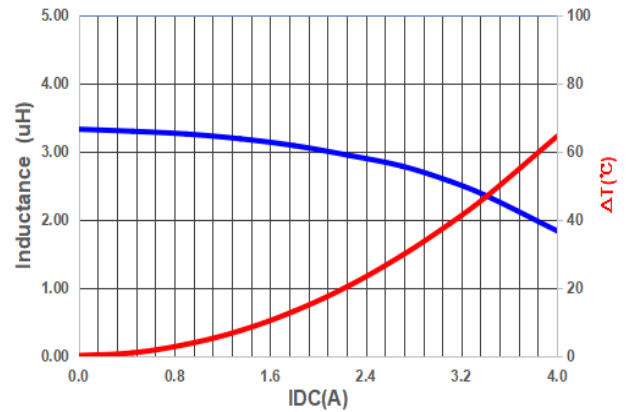
PIM322512A3R3M
