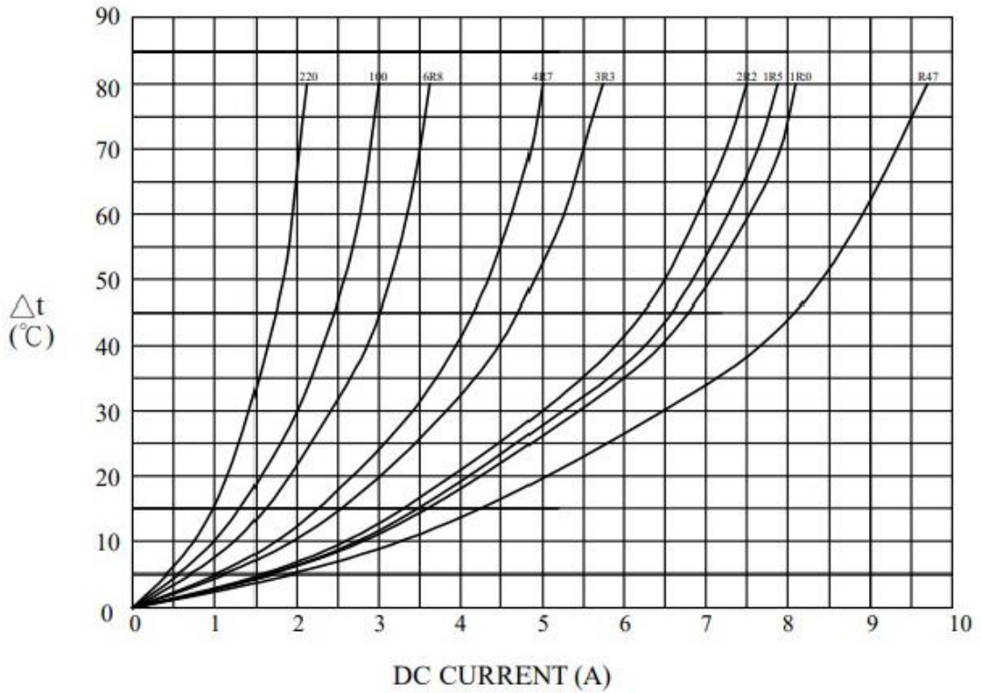
Temperature VS DC Current
