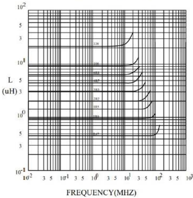
Inductance VS Frequency
