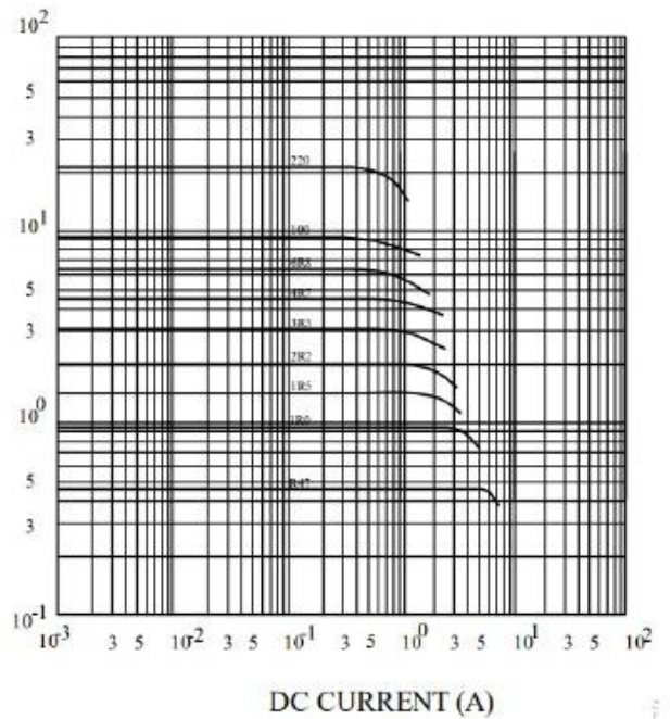
Inductance VS DC Current
