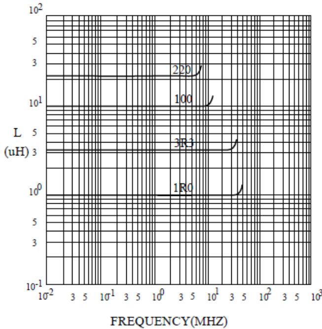
@ INDUCTANCE VS. FREQUENCY RESPONSE CURVE
