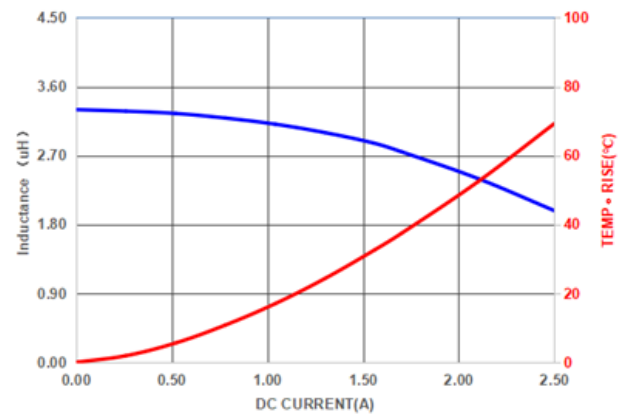
SPA252010RA3R3M
