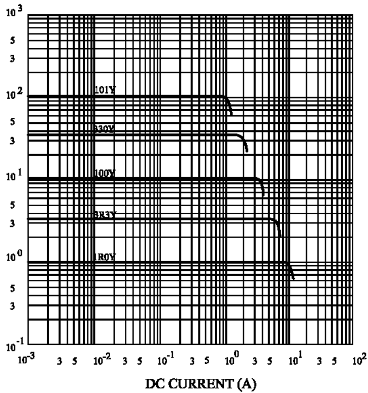
@ INDUCTANCE VS. DC SUPERPOSITION RESPONSE CURVE
